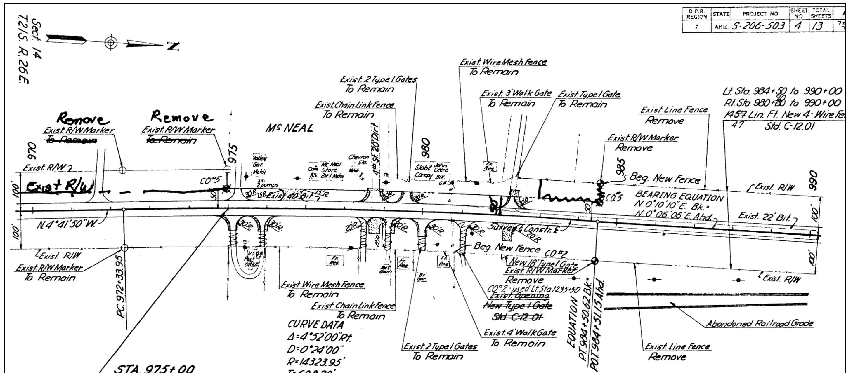
1974 As-Built sheet for the Douglas-Safford Highway (US 666) as it extends through McNeal, Cochise County, Arizona.
